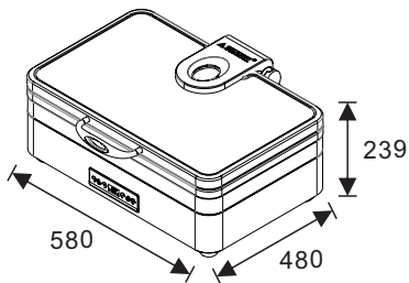
W07-1102T Induction Chafer W07-1101B Electrical Base Open Lid Height: 655mm
