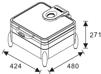
W07-2302T Induction Chafer W07-2304B Multi-Functional Base Open Lid Height: 687mm
