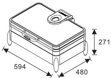
W07-1102T Induction Chafer W07-1104B Multi-Functional Base Open Lid Height: 687mm
